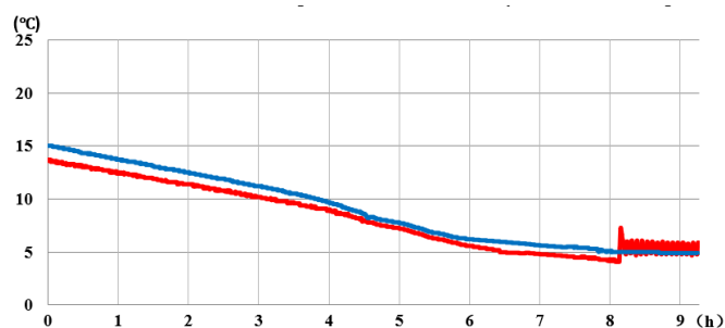
Variation of the water temperature in the container, while the ambient temperature is -10^\circ\text{C} , with a surface load of 0.05 \text{ W}/\text{cm}^2 (150W). It can be seen that the internal temperature of the container stabilizes at 5^\circ\text{C} .
