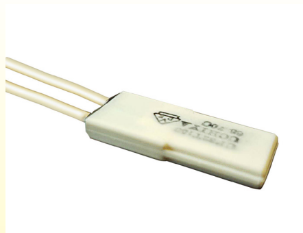
1980 ca Uchiya UP32 waterproof bimetallic limiter on Gitem private label heating blanket. (Ultimheat Collection)
