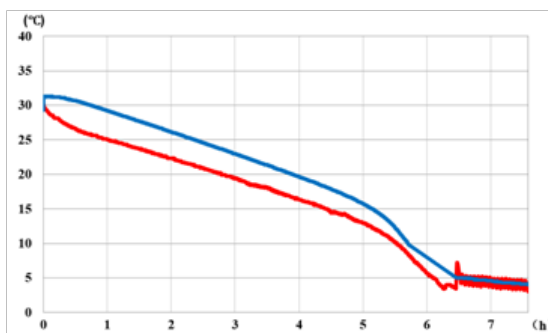
Variation of the water temperature in the container, while the ambient temperature is -35^\circ\text{C} , with a surface load of 0.1 \text{ W}/\text{cm}^2 (300W). It can be seen that despite the increased heating power, the internal temperature of the tank continues to fall slowly
